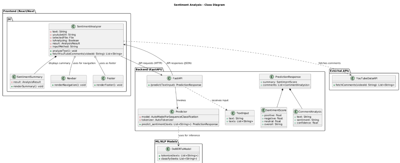
Figure 9: UML Diagram
